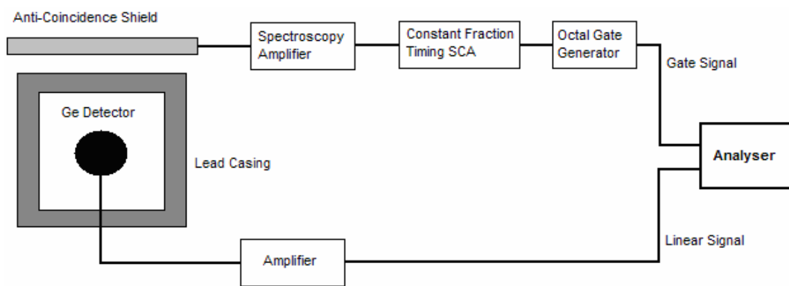
Fig. 11: Schematic diagram of the anti-coincidence shield and Ge detector.
