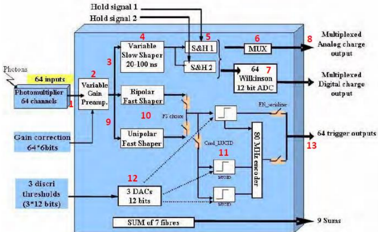
Figure 14.6. LEFT : MAPMT with full PMF mounted: MAPMT + isolator + spacer + voltage divider + spacer + isolator + passive board + active board. RIGHT : The layout of the MAROC 2. The figure is figure 3 in [58]. The red numbers are added to the figure.
