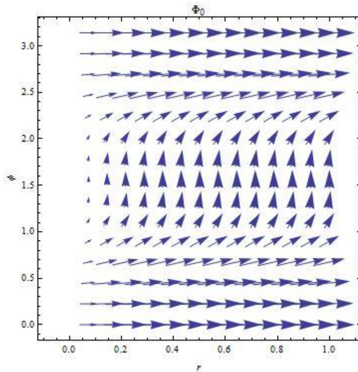
Fig1 : Standard Belavin-Polyakov soliton of topological charge 1
