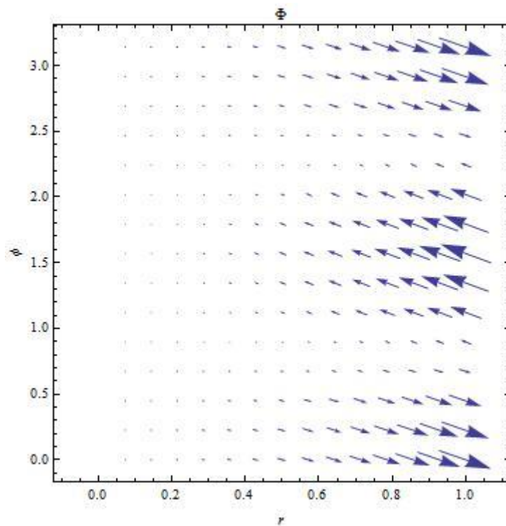
Fig2 : Topological soliton of charge 1 satisfying (nonlinear) Schrödinger equation
