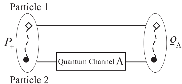
FIG. 3: A quantum channel \Lambda acting on one of the subsystems of a bipartite maximally entangled state of the form |\psi_+\rangle = \sum_k |k\rangle |k\rangle / \sqrt{d} . P_+ is the corresponding density operator, i.e. P_+ = |\psi_+\rangle \langle \psi_+| . The output is the state described by the density operator \varrho_\Lambda = \frac{1}{d} \sum_{kl} |k\rangle \langle l| \otimes \Lambda(|k\rangle \langle l|) , which contains a complete information about the channel. This isomorphism between \Lambda and \varrho_\Lambda allows to infer all properties of the channel from the corresponding properties of the state. Any subsequent estimations of \varrho_\Lambda , or any of its functions, provides information about the completely positive map \Lambda .
