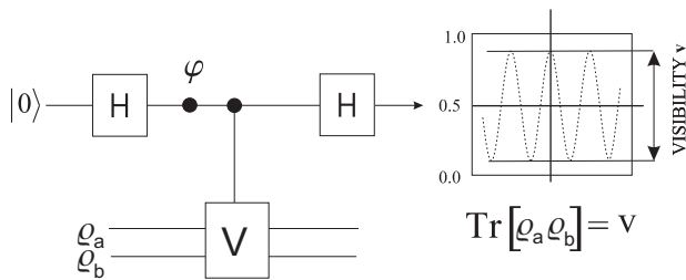
FIG. 2: A quantum network for direct estimations of both linear and non-linear functions of state. The probability of finding the control (top line) qubit in state |0\rangle at the output depends on the overlap of the two target states (two bottom lines). Thus estimation of this probability leads directly to an estimation of \text{Tr } \varrho_a \varrho_b = v = 2P_0 - 1 .
