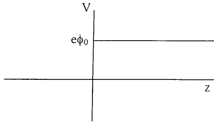
Fig. 1. The barrier potential associated with Klein's paradox.
